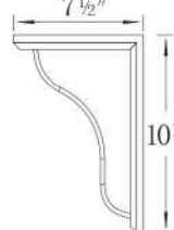
BRACKET
